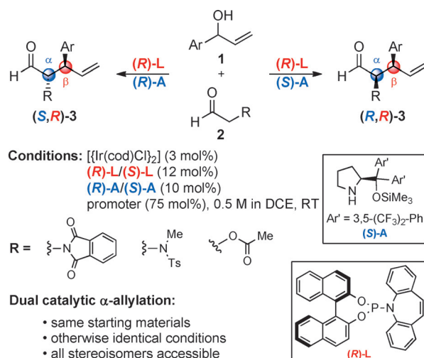
Scheme 1. Stereodivergent dual catalytic \alpha -allylation of protected \alpha -amino- and \alpha -hydroxyacetaldehydes. Ts = p -toluenesulfonyl; DCE = 1,2-dichloroethane.
